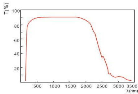
Transparency curve of LBO without coating
