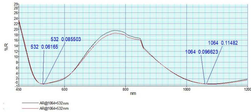
Transparency curve of LBO with AR coating @ 1064/532nm
